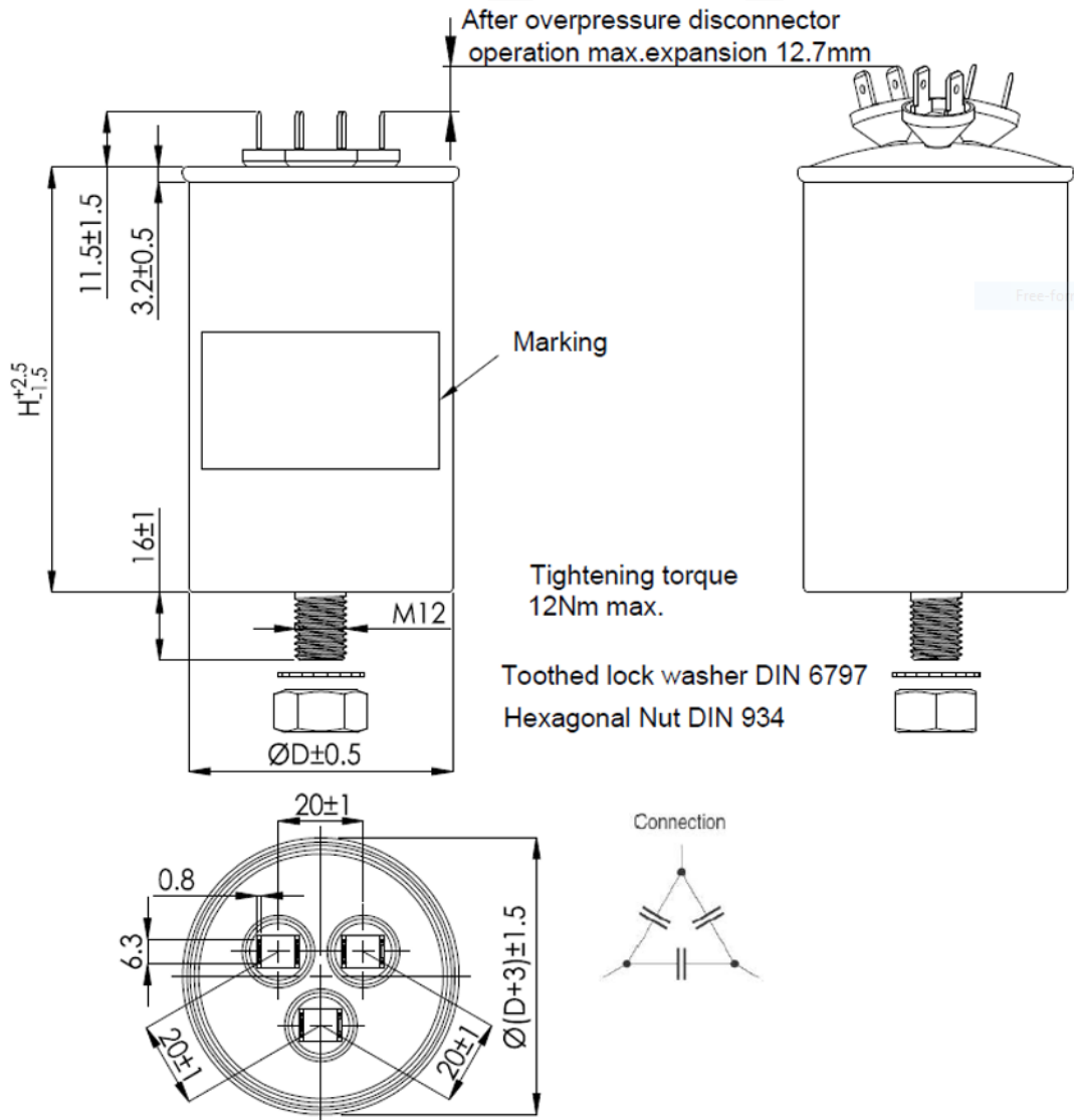
Figure 1: Series B32375* –fast-on terminal type A, delta connection
