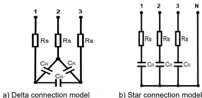
Figure 15: Resistance model of 3 Phase capacitor
