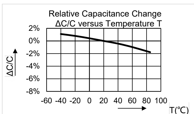
Figure 10: Temperature dependence of capacitance
