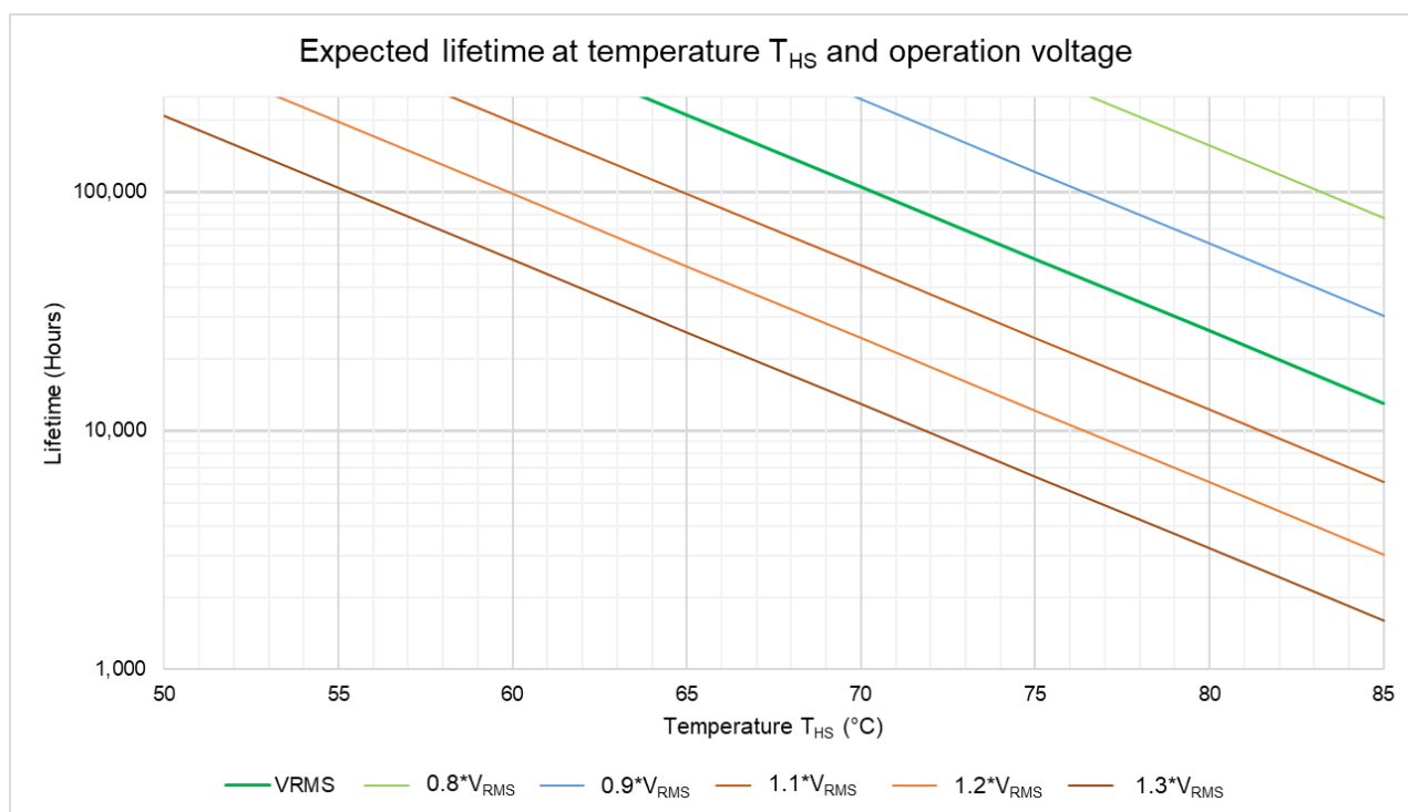
Figure 17: Expected lifetime in hours at different hotspot temperatures ( T_{HS} ) and voltages V_{RMS} .
