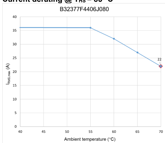
B32377F4406J080 Current derating @ T HS = 85 °C
