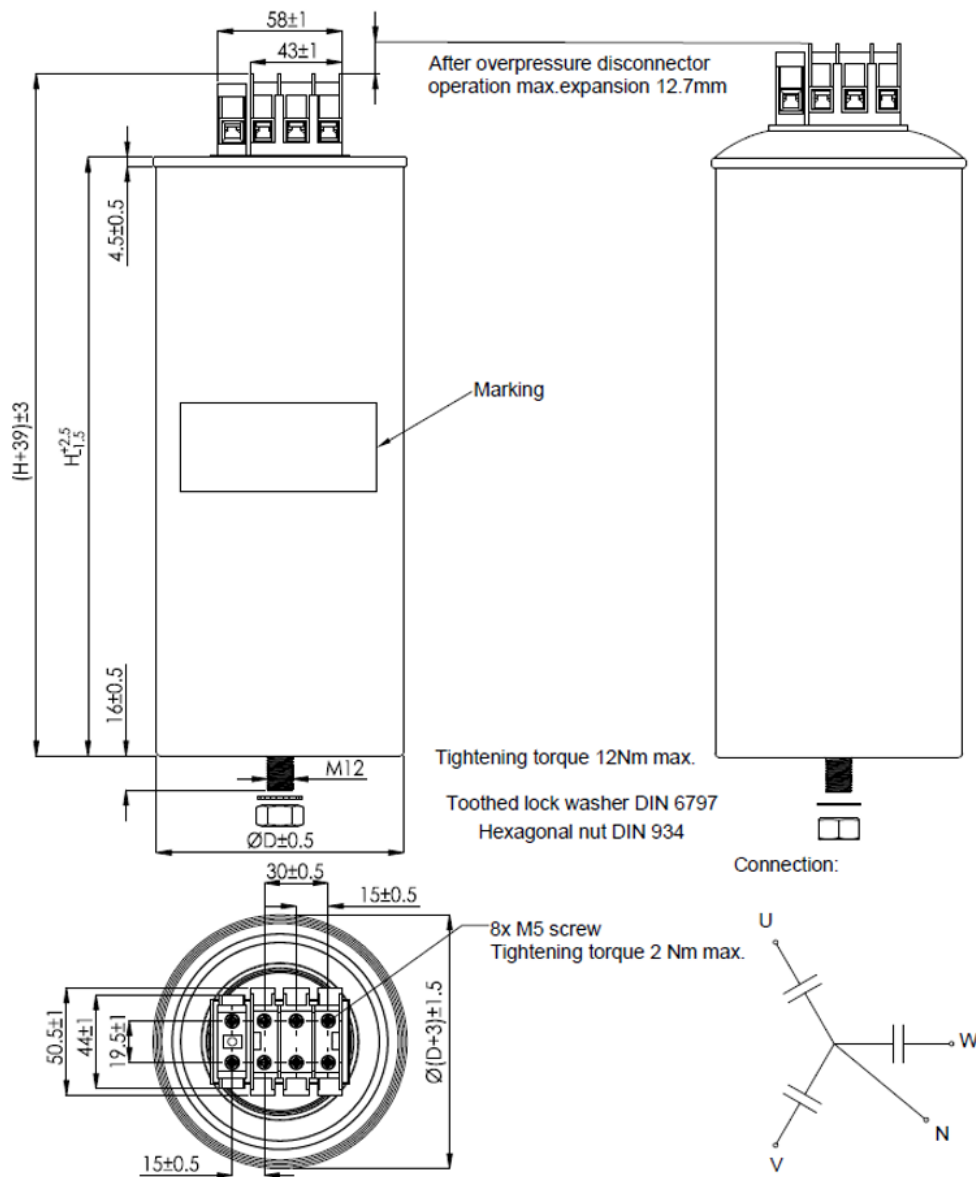
Figure 7: Series B32378* – M5 clamp terminal type E, star connection with neutral
