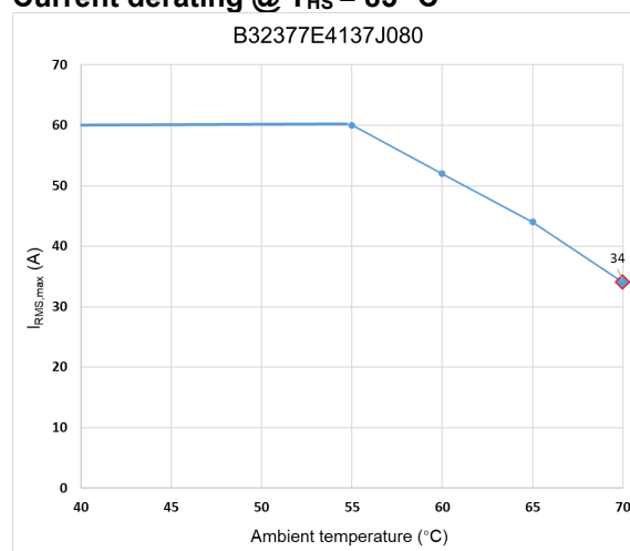
B32377E4137J080 Current derating @ T HS = 85 °C
