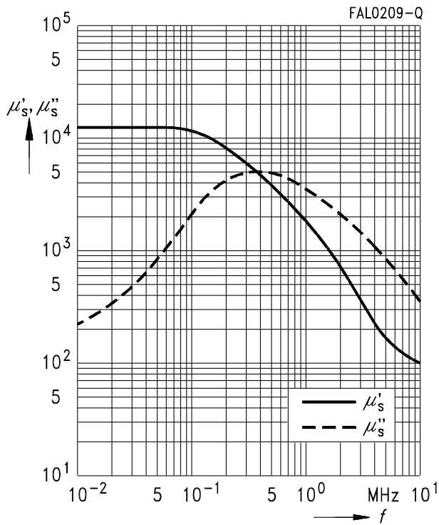
Complex permeability versus frequency (measured on R9.5 toroids, \hat{B} \leq 0.25 mT)
